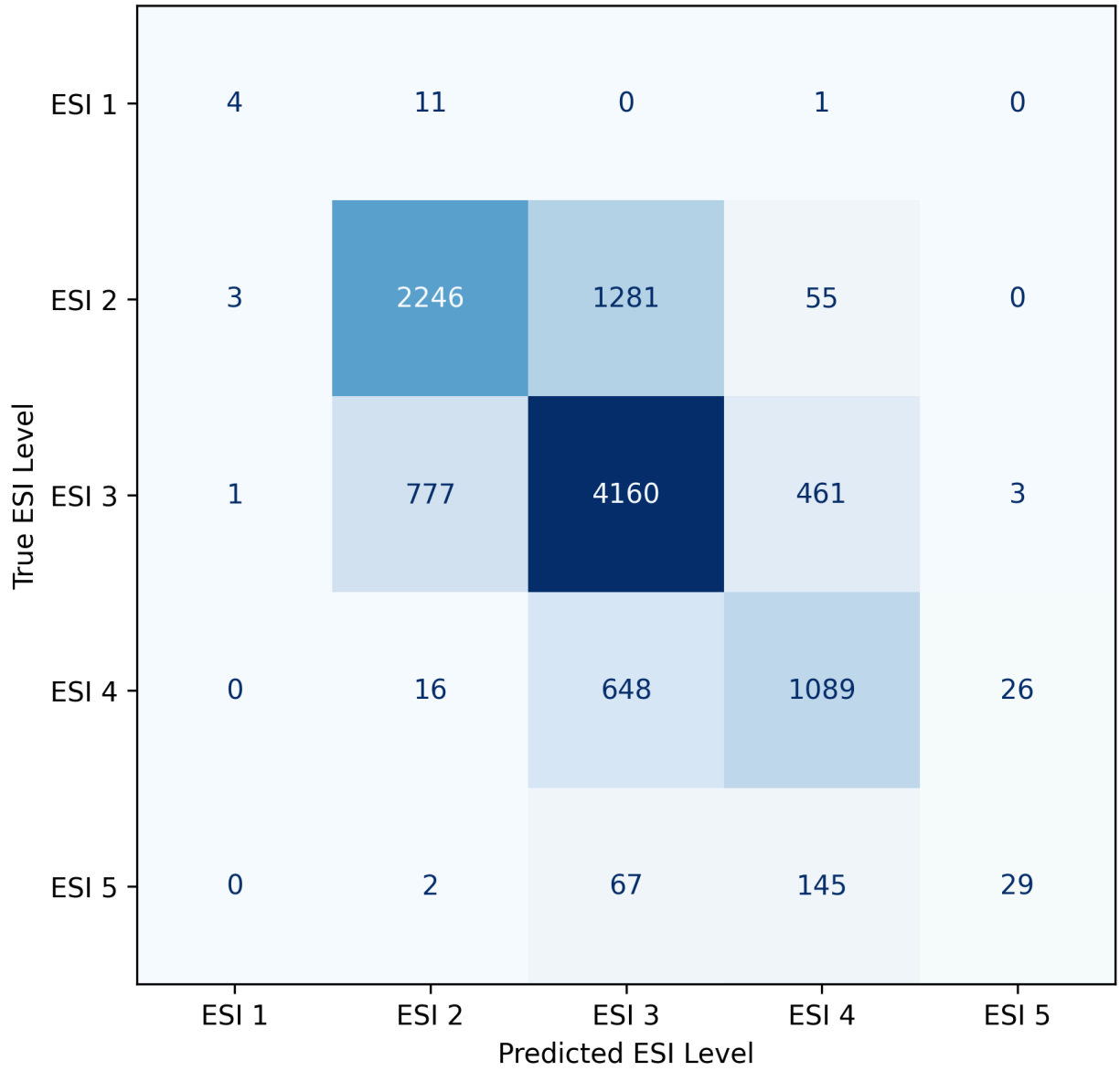
Refined Logistic Regression Confusion Matrix
