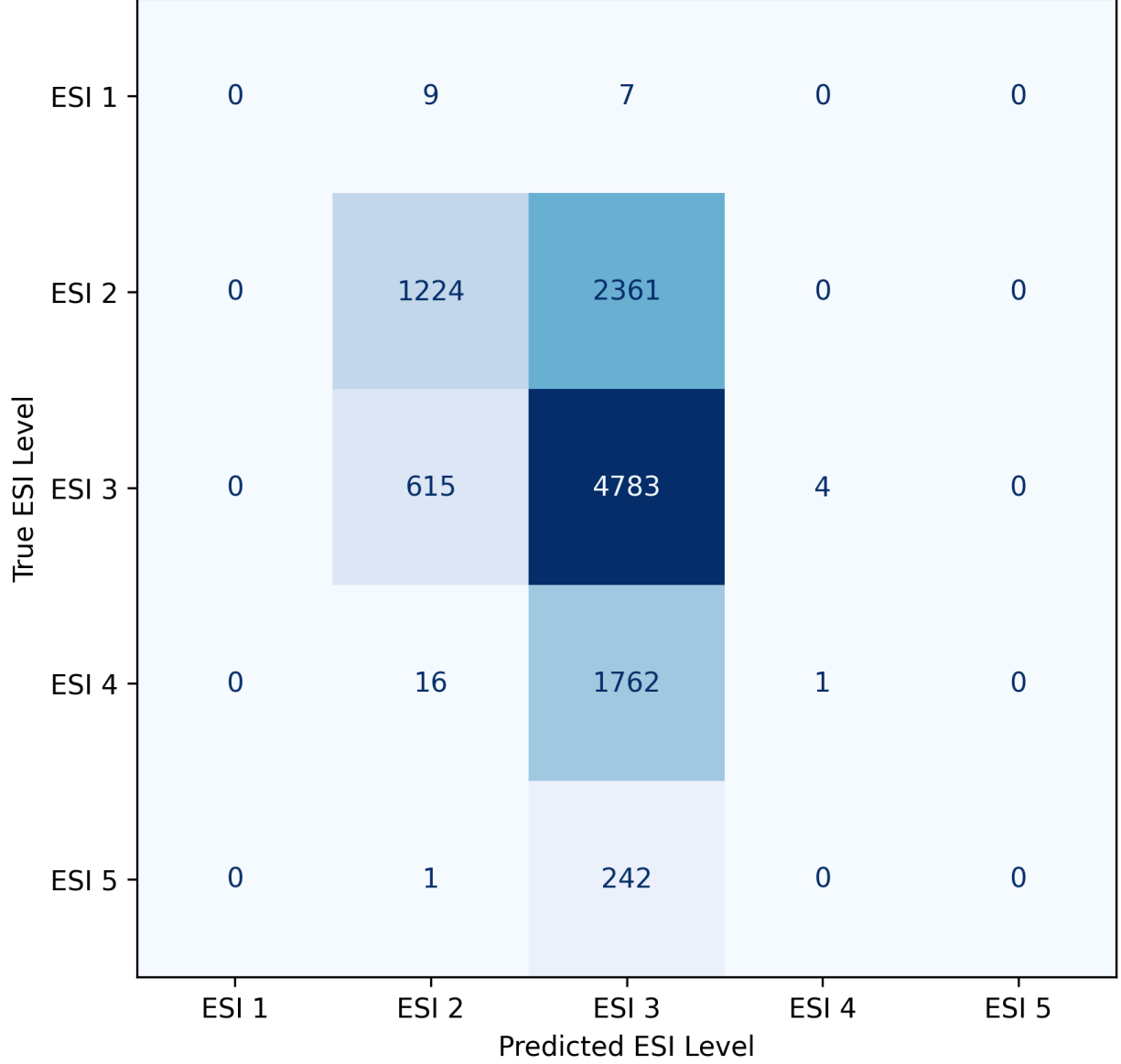
Logistic Regression Confusion Matrix
